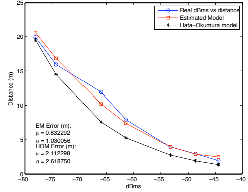
Fig. 5. Large-scale variations on propagation model
